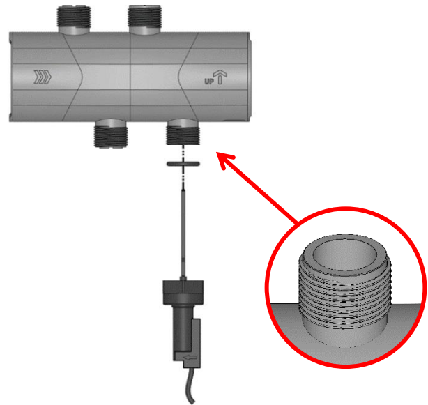
Flow sensor
